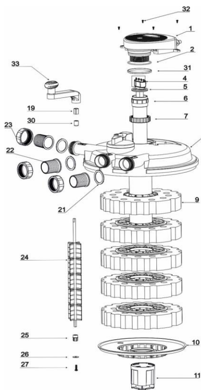
C VarioPress 24000/40000
